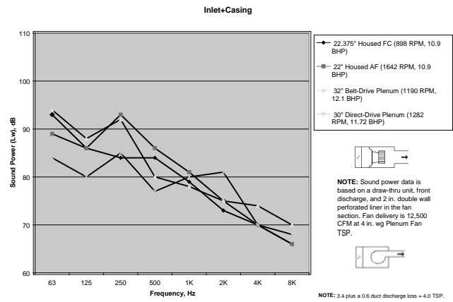
Figure 31. Comparison of inlet plus casing sound power by fan type
