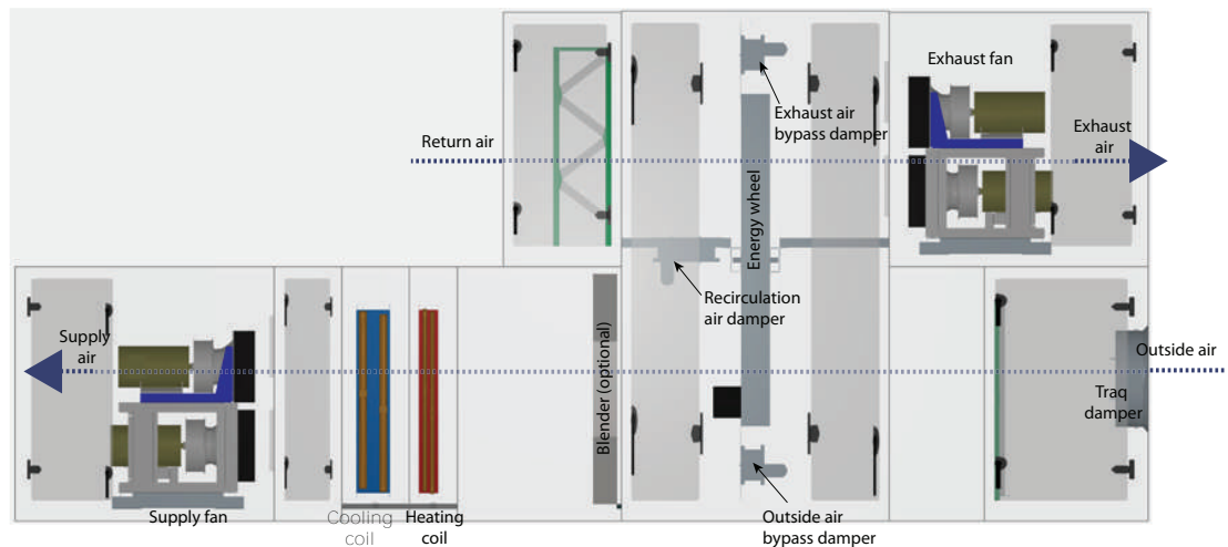
Figure 26. Energy-recovery with a total energy wheel in indoor unit
