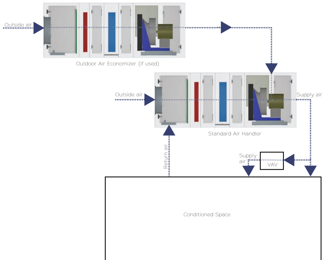
Figure 13. Dual-path design
