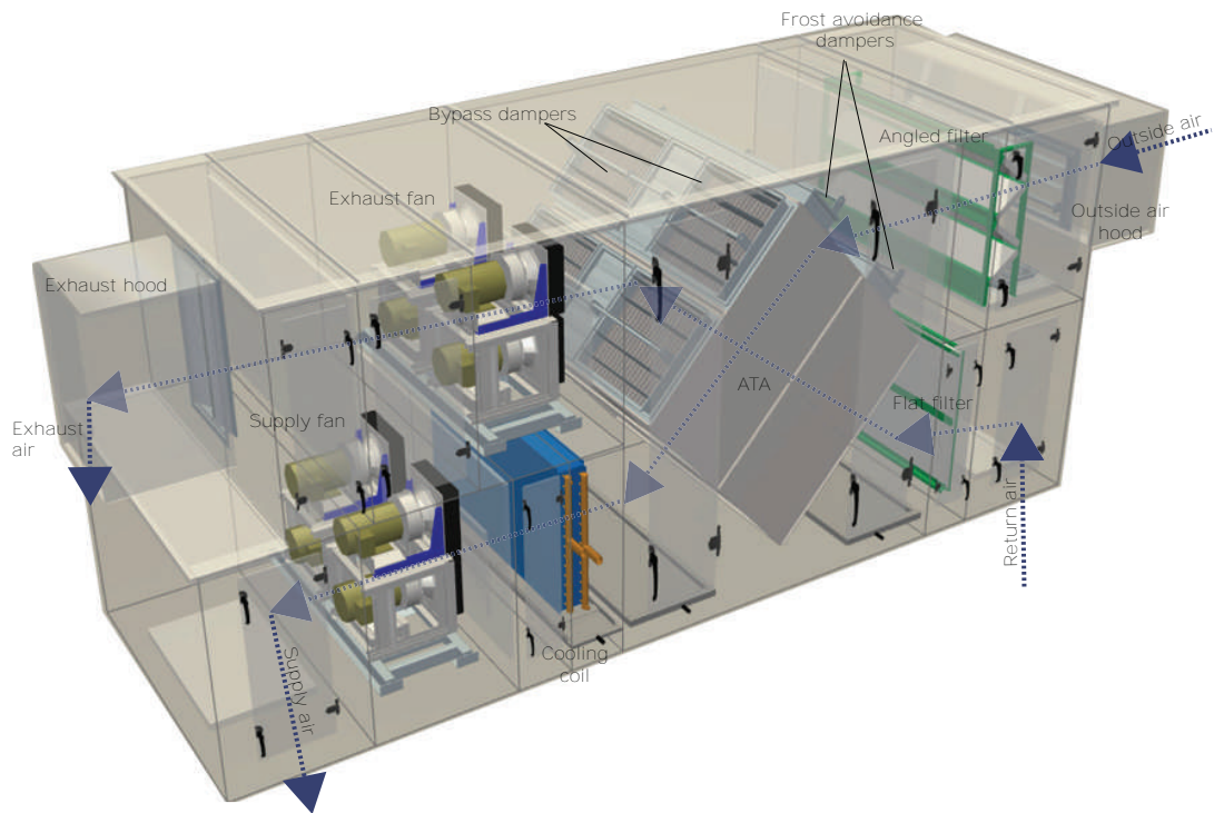
Figure 29. Energy recovery with air-to-air (ATA) plate frame heat exchanger
