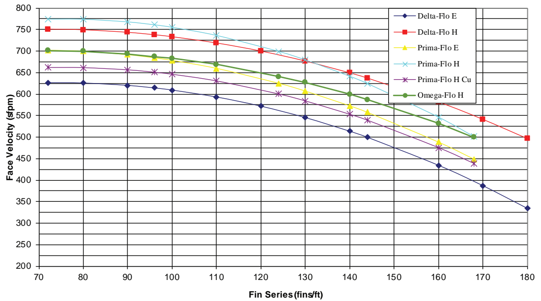
Figure 42. Face-velocity limits for moisture carryover with uncoated coils in unit size 12
