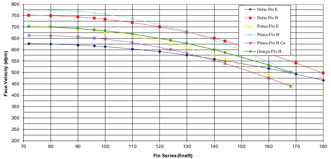
Figure 42. Face-velocity limits for moisture carryover with uncoated coils in unit size 12
