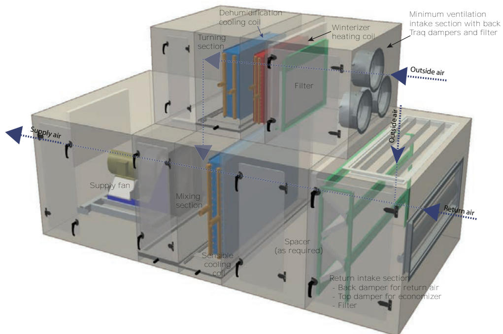
Figure 23. Horizontal indoor SDU
