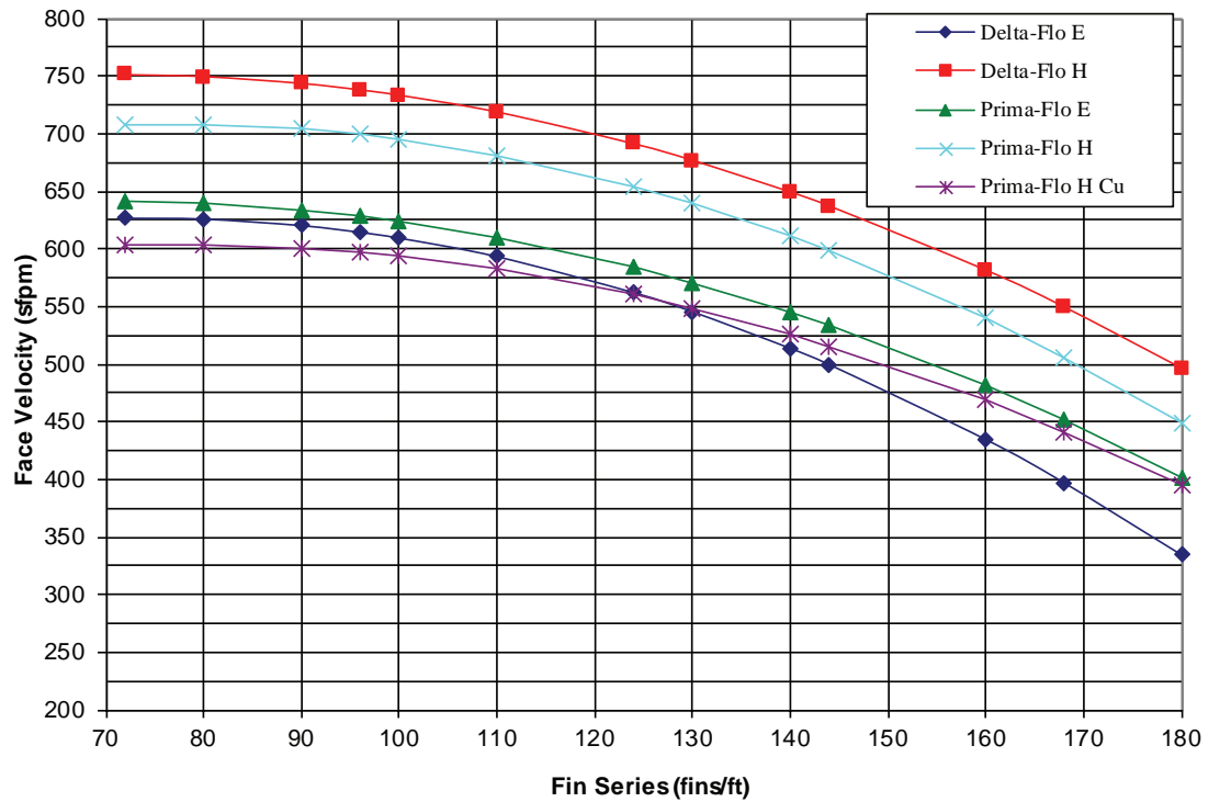
Figure 46. Face velocity limits for moisture carryover with uncoated coils in unit sizes 50-57
