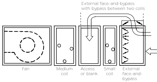
Figure 38. Configuration A
