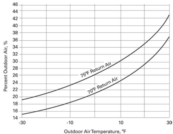
Figure 33. Blender performance with 55°F leaving air temperature
