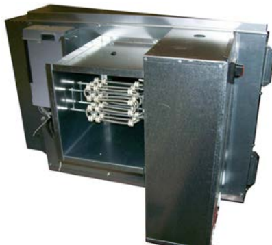
Figure 37. Typical blow through heater
