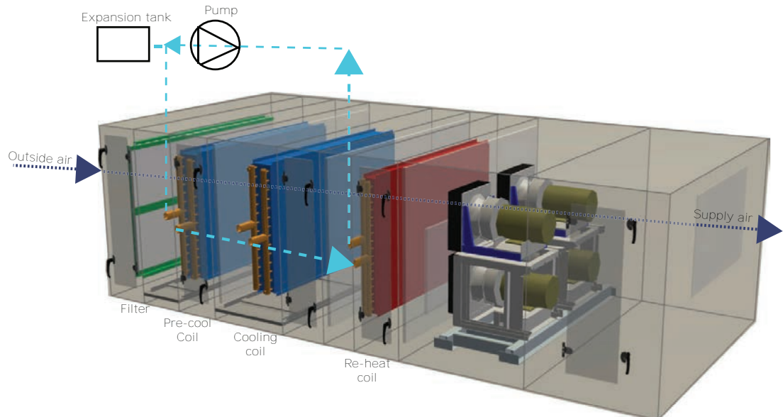
Figure 22. Series dehumidification with coil run-around loops
