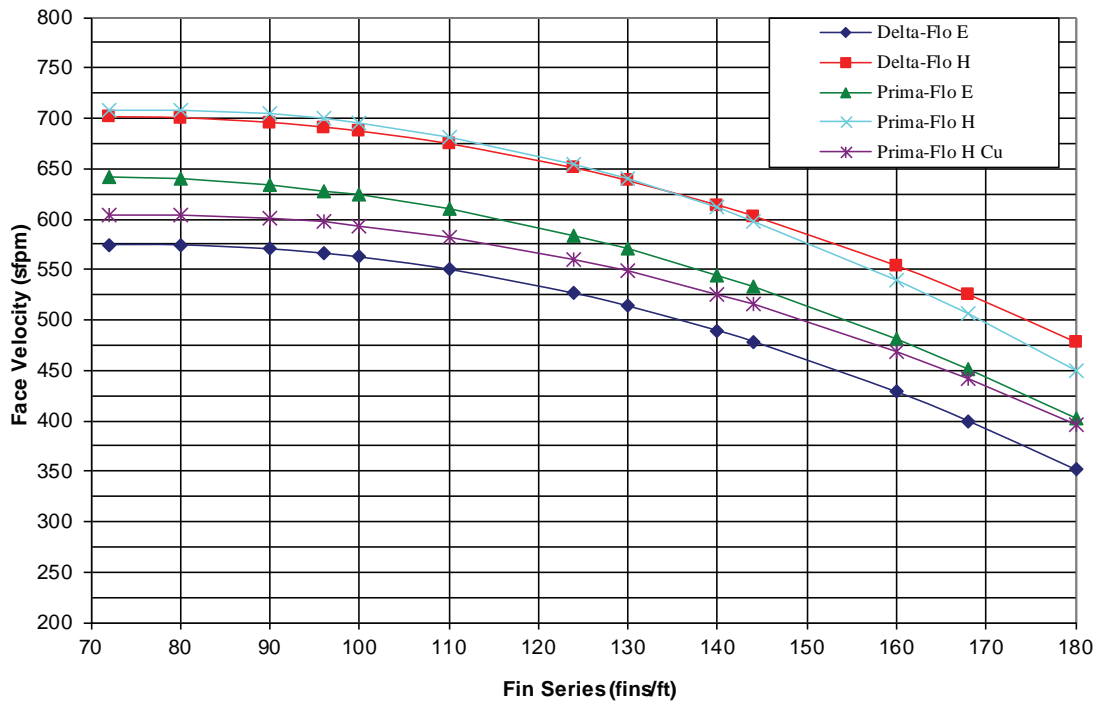
Figure 48. Face velocity limits for moisture carryover with uncoated coils in unit size 88-120
