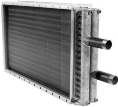
Figure 34. Coil with copper header
