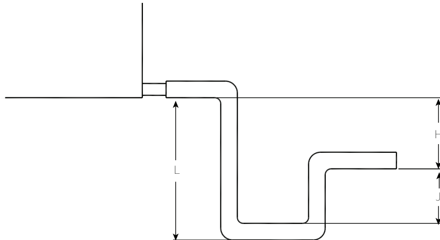
Figure 10. Drain pan trapping for positive and negative pressure applications
