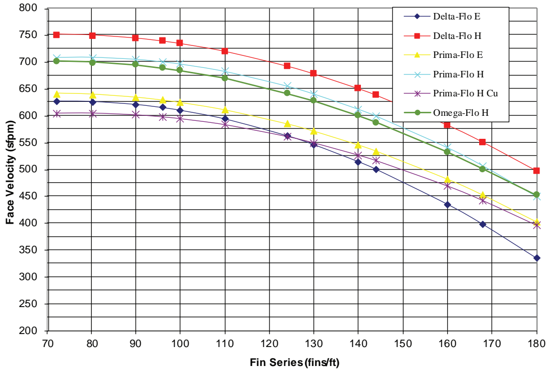
Figure 44. Face-velocity limits for moisture carryover with uncoated coils in unit sizes 21-30
