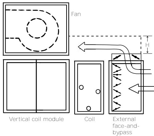
Figure 40. Configuration C
