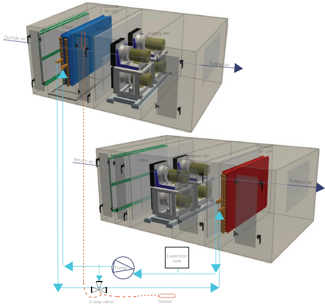
Figure 28. Energy recovery with a runaround coil loop
