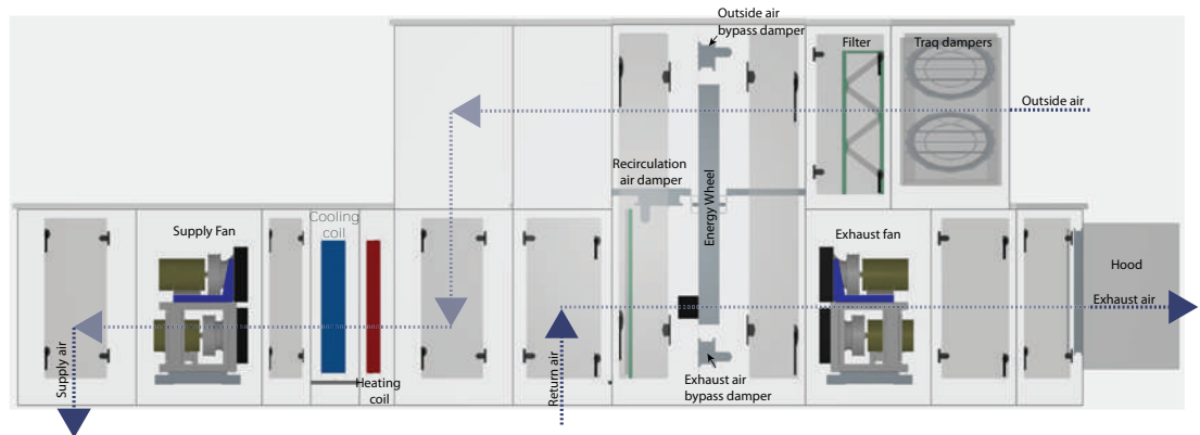
Figure 27. Energy-recovery with a total energy wheel in outdoor unit
