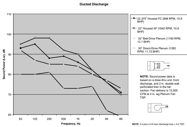
Figure 30. Comparison of discharge sound power by fan type
