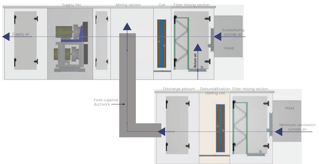
Figure 25. Dehumidifying with two outdoor SDUs
