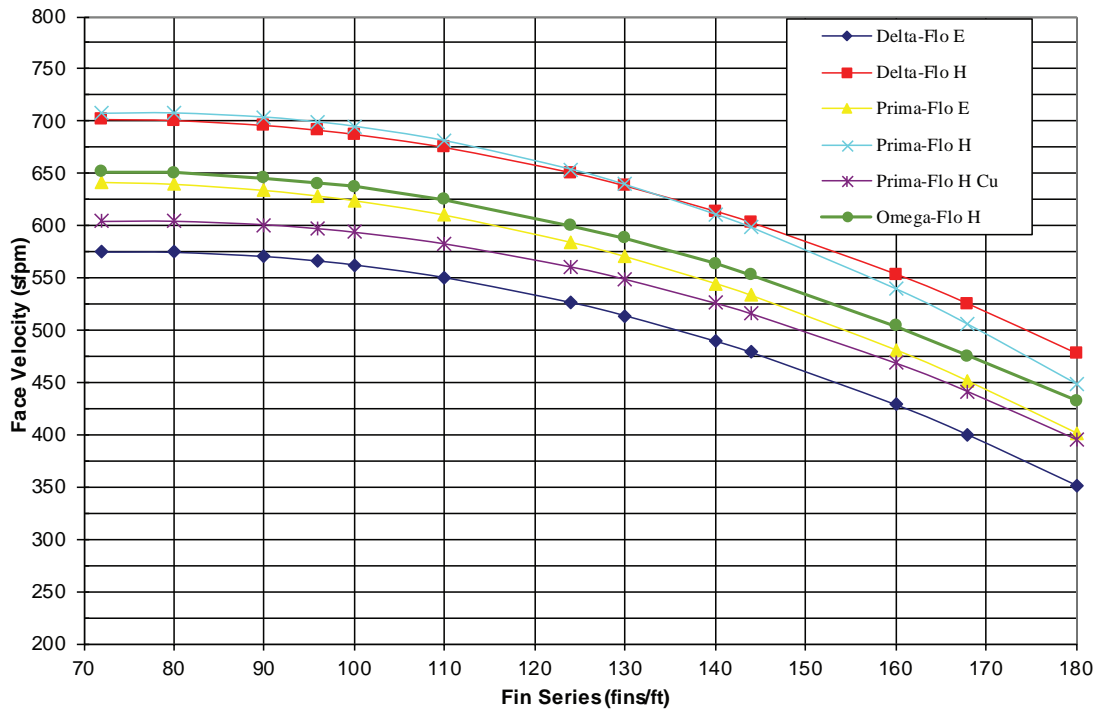
Figure 44. Face-velocity limits for moisture carryover with uncoated coils in unit sizes 21-30
