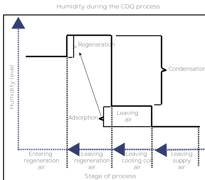
Figure 21. Humidity levels during the dehumidification process
