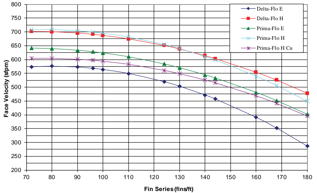
Figure 46. Face velocity limits for moisture carryover with uncoated coils in unit sizes 50-57
