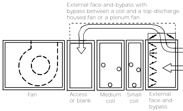
Figure 40. Configuration C
