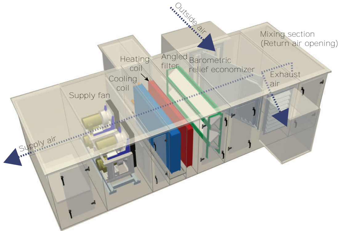
Figure 19. Building pressurization with a barometric relief economizer arrangement
